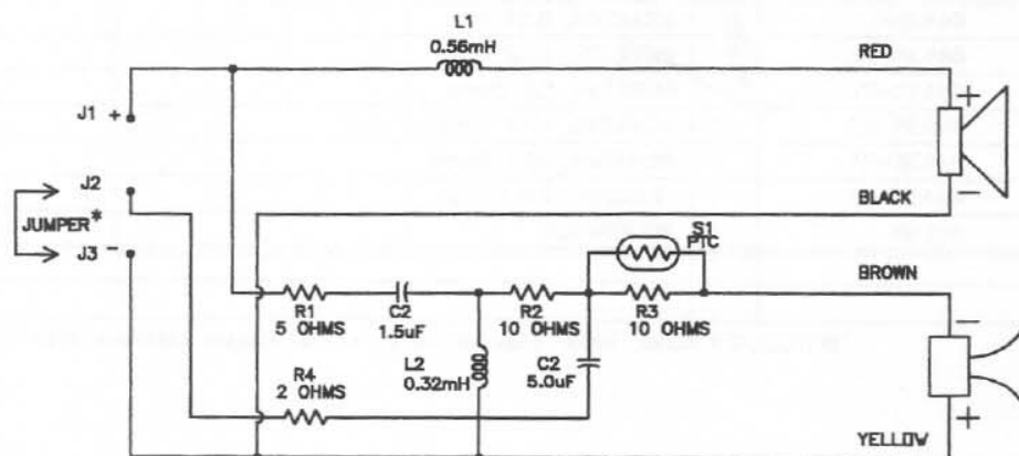
WIRING DIAGRAM
